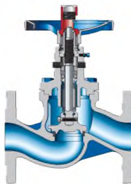
VOA®-H EN-GJL-250
