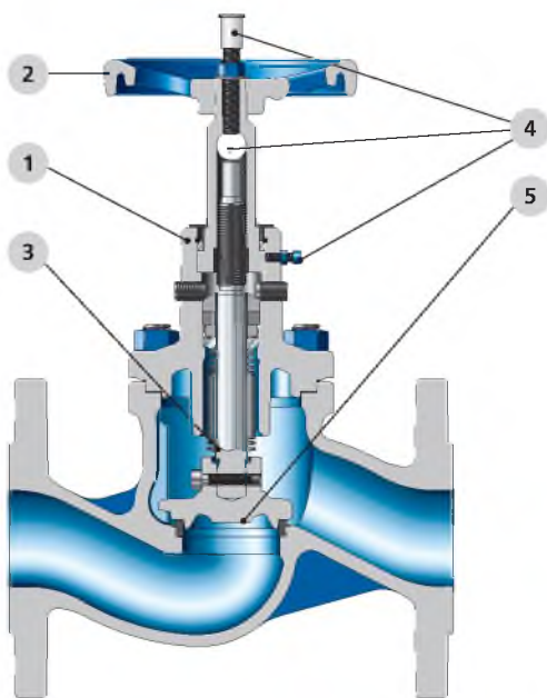
VOA®-H EN-GJS-400-18-LT
